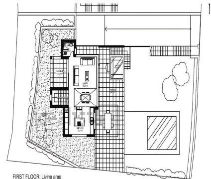
FIRST FLOOR: Living area 72,00 m 2 BUILT
